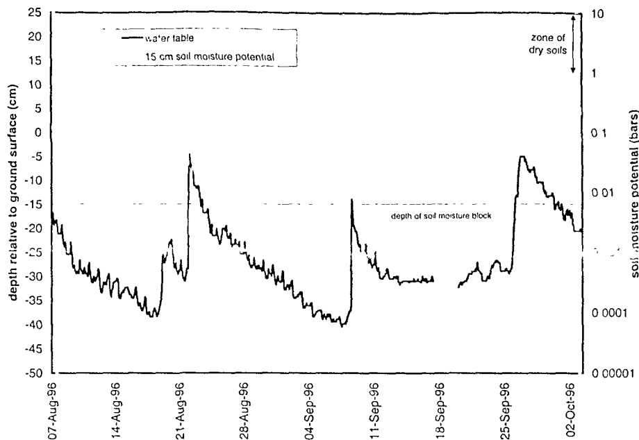
Figure 5. Soil-moisture potential and water-table hydrograph for the late 1996 growing season. The only deviations from baseline saturated conditions occur when the water table rises into the root zone where the soil moisture probe is located.
