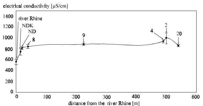
Fig. 7: Variations of the specific electric conductivity in groundwater along the hydrochemical profile (confidence of means with 95% level of significance).
