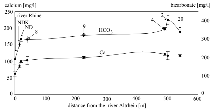
Figure 10. Variations of bicarbonate and calcium concentrations in groundwater along the hydrochemical profile.
