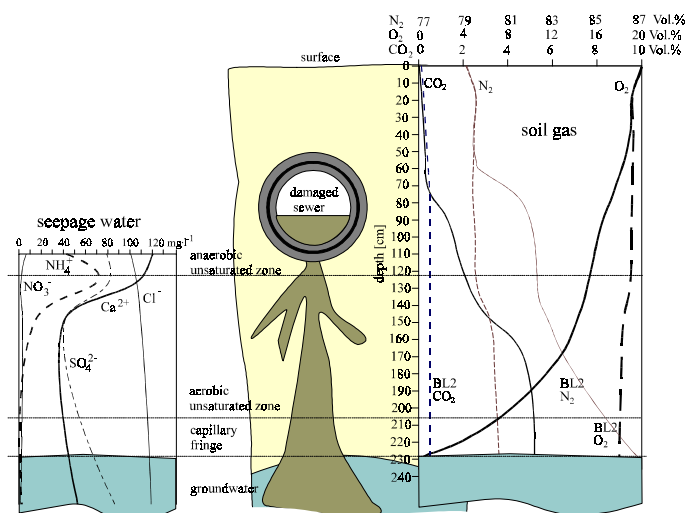
Figure 12. Variations in waste water chemistry and soil gas composition during the effluent seepage through the subsurface below a damaged sewer
