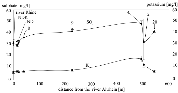
Figure 8. Variations of sulphate and potassium concentrations in groundwater along the hydrochemical profile.
