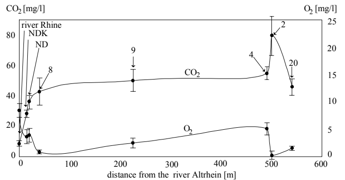
Figure 11. Variations of carbon dioxide and oxygen concentrations in groundwater along the hydrochemical profile.
