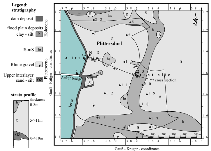
Figure 3. Schematic local geological map of Plittersdorf and location of groundwater observation wells.
