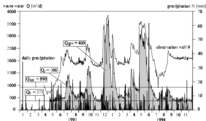
Figure 13. Waste water discharge and daily precipitation at the sewage pumping station in Plittersdorf for 1993 and 1994 ( Q_{\text{tot}} = total discharge; Q_r = storm water runoff, Q_h = runoff from households; Q_{\text{gw}} = groundwater infiltration).
