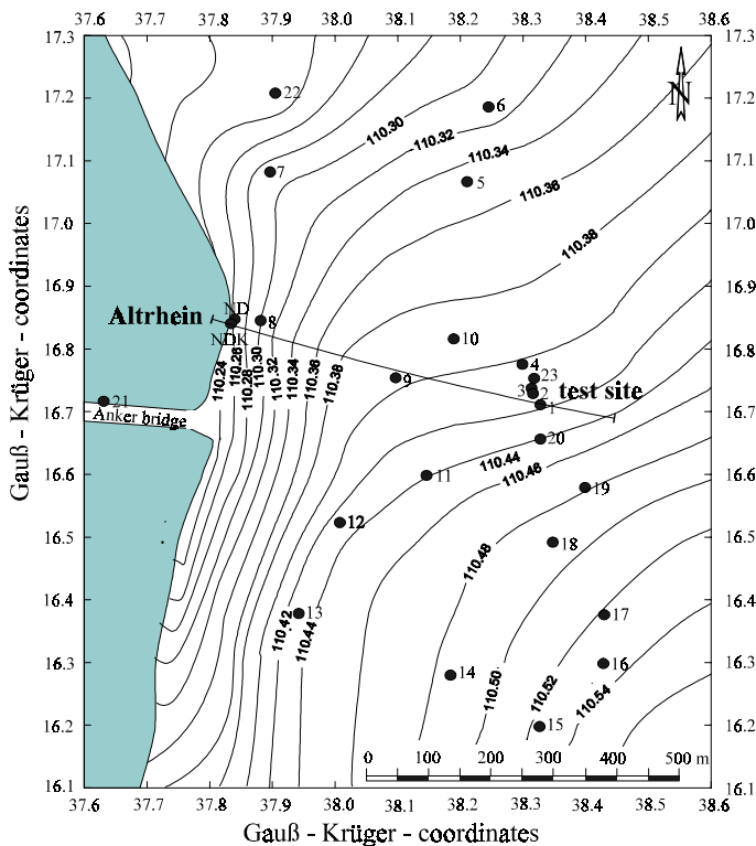
Figure 5. Map of groundwater level in Plittersdorf during low river water level on 10.11.1993 [m a.s.l.].
