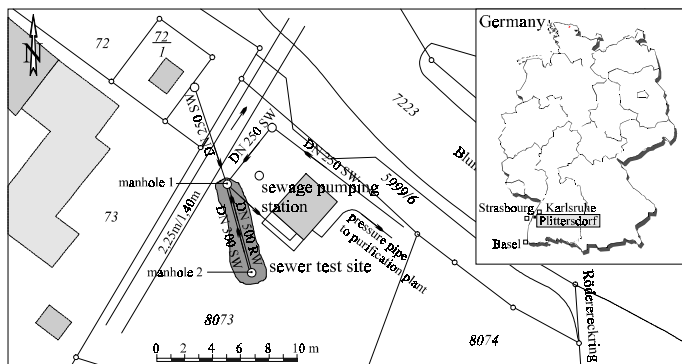
Figure 6. Location of waste water test site in Plittersdorf (Southern Germany).
