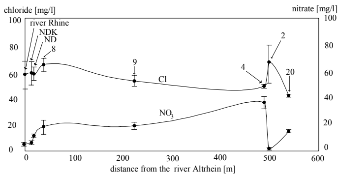
Figure 9. Variations of chloride and nitrate concentrations in groundwater along the hydrochemical profile.
