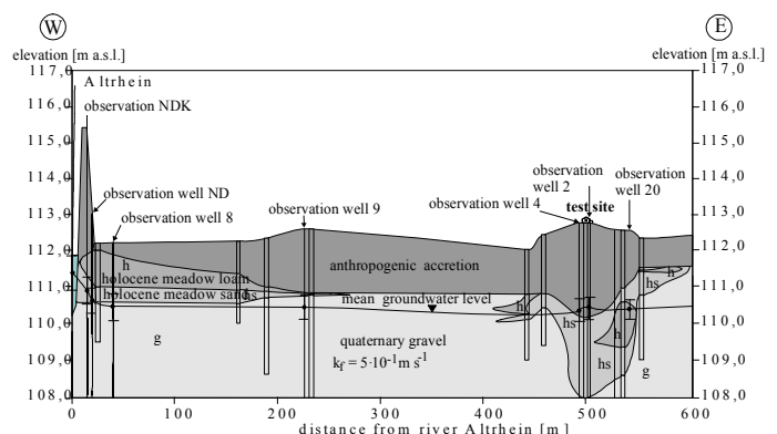
Figure 4. Schematic geological cross section (location is indicated in Figure 3).
